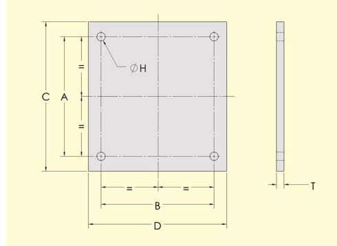
Dimension table for location plates to suit BY products
