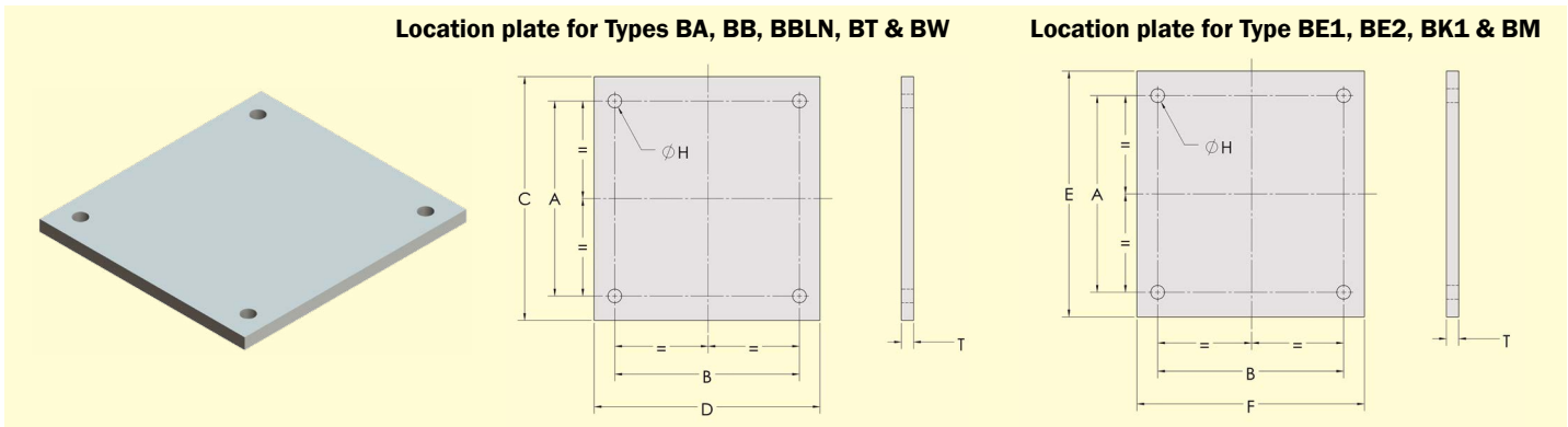
Dimension Table for BeamClamp® Location Plates
